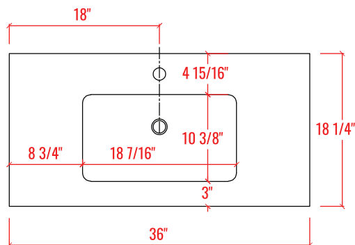
ELEVATION VIEW
